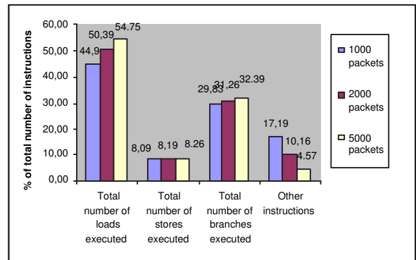
Fig. 3. Instruction Distribution
